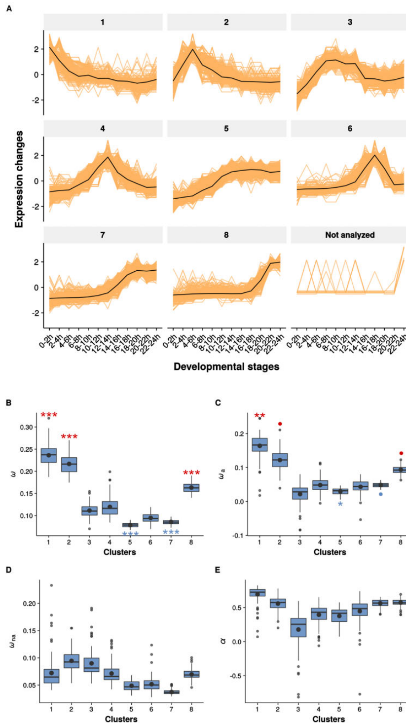
FIG. 2. —Clusters of temporal profiles of expression of embryonic development genes and their \omega_{ar} , \omega_{na} , and \omega estimated using DFE-alpha. (A) Temporal expression profile for all the genes belonging to each cluster. (B) \omega for each cluster. (C) \omega_a sampling for each cluster. (D) \omega_{na} for each cluster. (E) \alpha for each cluster. Each point in the plots in (B)–(E) is calculated for a randomly drawn sample of the set of genes in each cluster with replacement (100 bootstrap replicates per cluster). Asterisks represent the significance by a permutation test, the color indicates whether the value was higher (red) or lower (blue) than expected ( \bullet , 0.1-0.05 , * < 0.05 , ** < 0.01 , and *** < 0.001 ). Number of genes analyzed in supplementary table S1, Supplementary Material online. Permutation P values are shown in supplementary table S12, Supplementary Material online.
